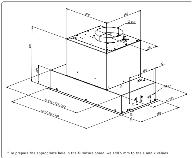
MINIMAL 7 - 55 cm / 74 cm / 90 cm
