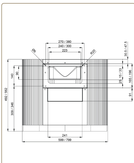
MONO 60/80 - REAR
