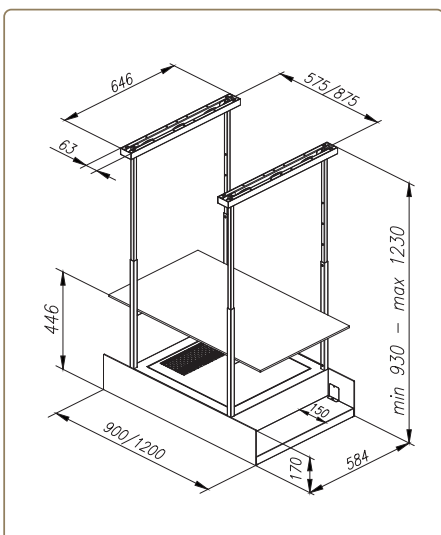
MINIMAL 1 - 90 cm / 120 cm
