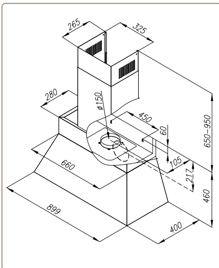
MINIMAL 6 - 90 cm
