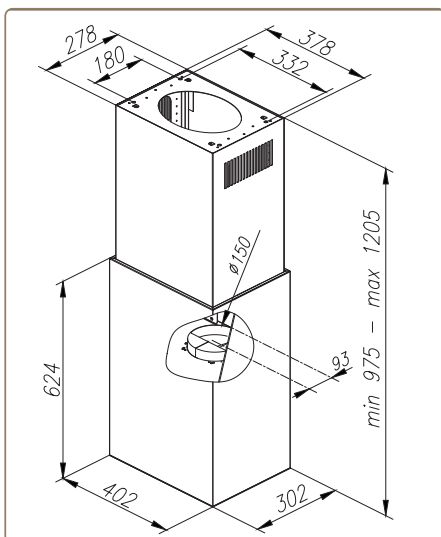
CUBE W
