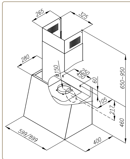
MINIMAL 5 - 60 cm / 90 cm
