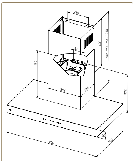
MINIMAL 8
