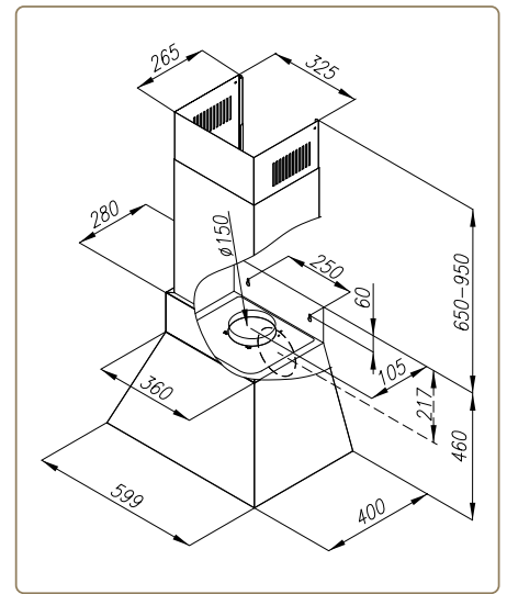
MINIMAL 6 - 60 cm
