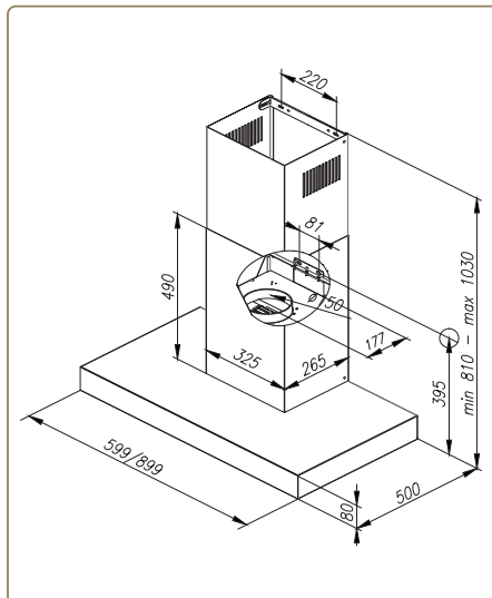
T LIGHT - 60 cm / 90 cm
