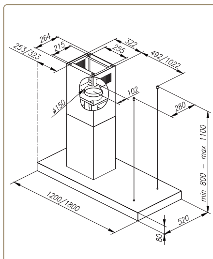
MINIMAL 2 - 120 cm / 180 cm
