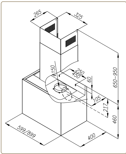
MINIMAL 4 - 60 cm / 90 cm
