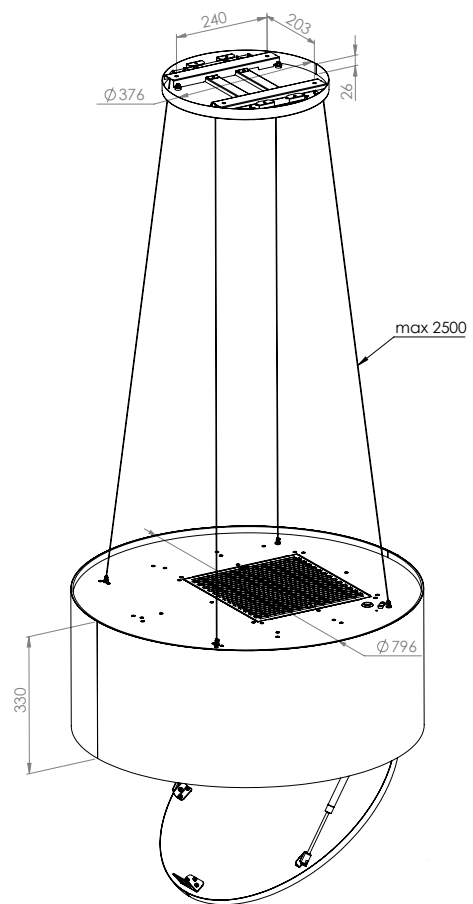
PIU LIGHT / 80 CM
