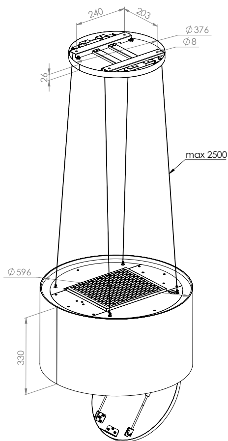
PIU LIGHT / 60 CM
