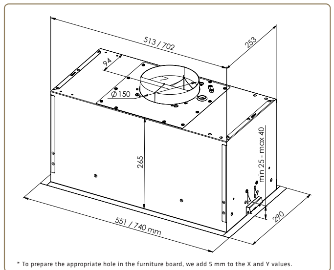
DUO - 55 / 74 cm
