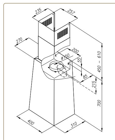
MINIMAL 3
