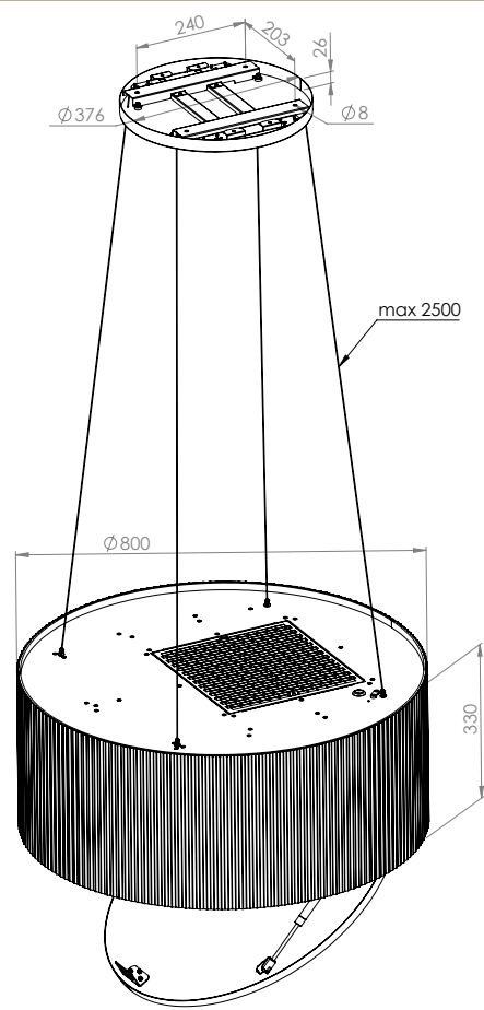
MONO LIGHT / 80 CM
